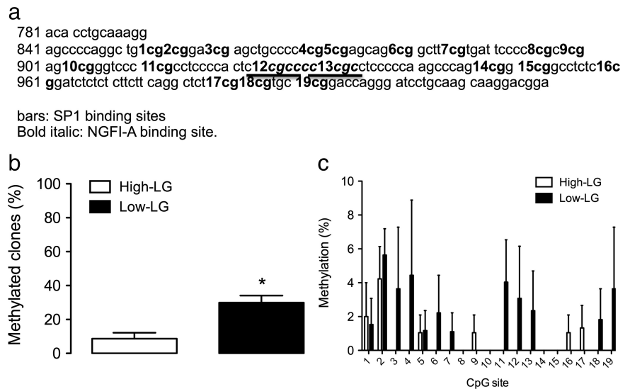
Figure 4. Maternal effect on GAD1 promoter methylation. a , A sequence map of the GAD1 promoter showing the NGFI-A consensus sequence. b , Mean \pm SEM percentage of cloned GAD1 promoter sequences revealing one or more methylated CpG sites as determined using NaBis mapping (10–20 clones per sample, with n = 5 /group; * p < 0.01 ). c , Mean \pm SEM percentage of cloned GAD1 promoter sequences revealing one or more methylated CpG sites as determined using NaBis mapping for each of the individual CpG dinucleotides within the GAD1 promoter region. Statistical analysis reveals an overall group effect.
