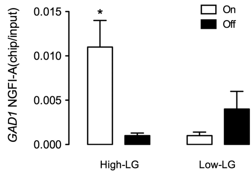
Figure 2. Maternal regulation of NGFI-A binding to the GAD1 promoter. Mean \pm SEM qPCR data of the amplified GAD1 promoter sequence from NGFI-A immunoprecipitated hippocampal extract as a ratio of that from the input fraction. Hippocampal samples were obtained from the male, postnatal day 4 pups of high- or low-LG mothers immediately after a nursing bout (ON) or 25 min after the termination of a nursing bout (without any subsequent mother-pup interaction; OFF; n = 4-6 /group; * p < 0.05 from all other groups).
