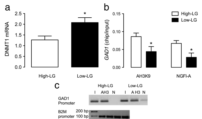
Figure 5. Maternal regulation of the epigenetic state of the GAD1 promoter. a , Mean \pm SEM levels of DNMT1 mRNA quantified using qRT-PCR analysis of the amplified DNMT1 mRNA (relative to the \beta 2M standard) in hippocampal samples derived from adult offspring of high- or low-LG mothers ( n = 5 /group; * p < 0.05 ). b , Mean \pm SEM qPCR data of the amplified GAD1 promoter sequence immunoprecipitated from hippocampal samples with an antibody to H3-K9ac or NGFI-A and normalized to the input values (* p < 0.05 ; n = 4 samples/group). c , Representative images of GAD1 and \beta 2M qPCR products on agarose gel confirming the amplification of a single specific product from chromatin immunoprecipitation assays described above.
