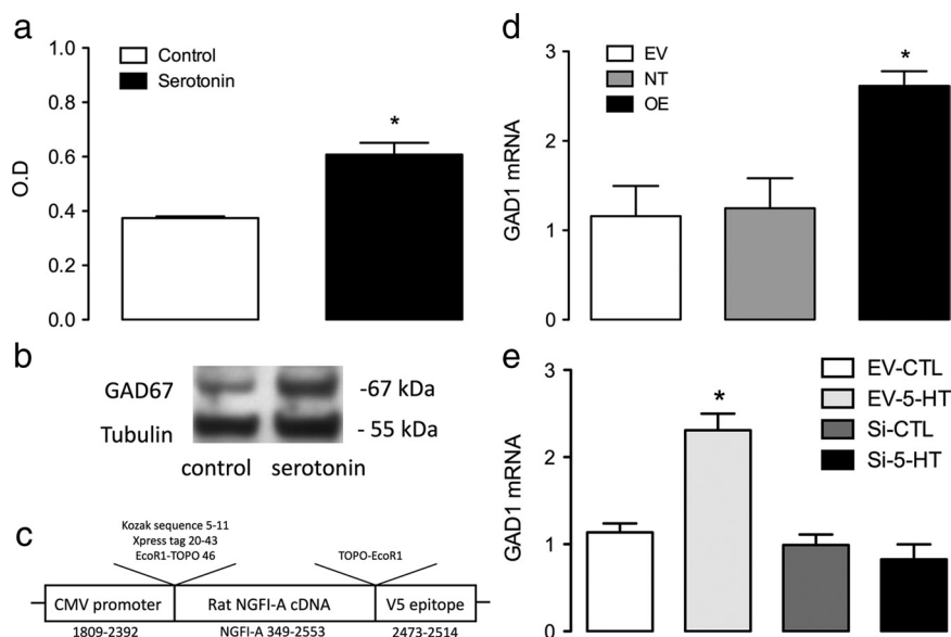
Figure 3. Regulation of GAD1 expression in primary hippocampal neuronal cell cultures. a , Mean \pm SEM levels of GAD 67 expression (relative optical density) quantified using Western blotting with samples from hippocampal cultures treated with serotonin (5-HT) (1 \mu M) or medium alone ( *p < 0.01 ). b , Representative Western blots showing bands corresponding to GAD 67 and \alpha -tubulin (used to control for loading variation). c , Physical map of the CMV/V5-His-NGFI-A expression vector. d , Mean \pm SEM levels of GAD1 mRNA quantified using qRT-PCR analysis of the amplified GAD1 mRNA (relative to the \beta 2M standard) in primary hippocampal neuronal cultures treated with a lentiviral vector containing an NGFI-A expression plasmid (OE), the empty viral vector (EV), and a reference, no-treatment group (NT) ( n = 8 /group; *p < 0.05 ). e , Mean \pm SEM levels of GAD1 mRNA amplified from primary hippocampal neuronal cultures, quantified using qRT-PCR (with \beta 2M as standard), treated with medium alone plus empty viral vector (EV-CTL), 5-HT in medium plus empty viral vector (EV-5-HT), medium alone plus the viral vector containing an NGFI-A siRNA (Si-CTL), and 5-HT in medium plus the viral vector containing an NGFI-A siRNA (Si-5-HT; n = 4-6 /group) in sample ( *p < 0.01 compared with all other groups).
